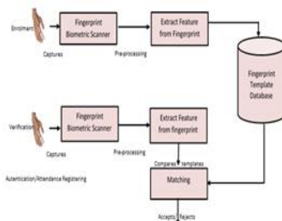
Fig. 1 Architecture of BFASSM authentication system
