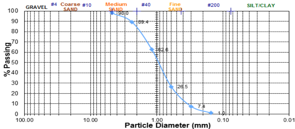
Fig. 1: Particle Size Distribution Curve of Fine Aggregates
