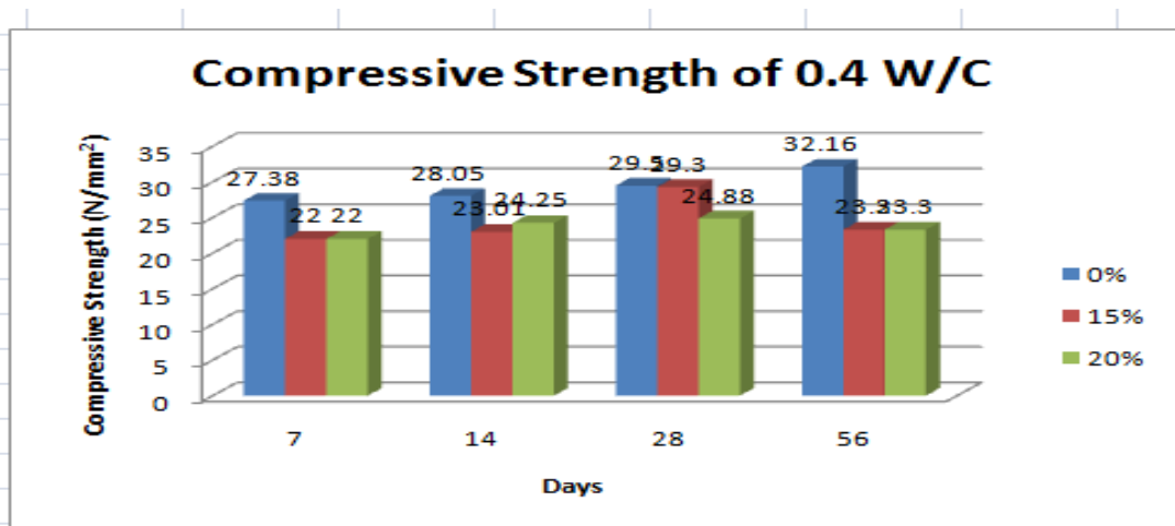
Fig. 4: Graph of compressive strength of concrete of w/c of 0.4 with curing days.
