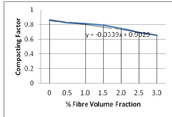
Graph 2: Compacting Factor Test
