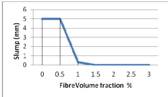
Graph 1: Slump test (mm)
