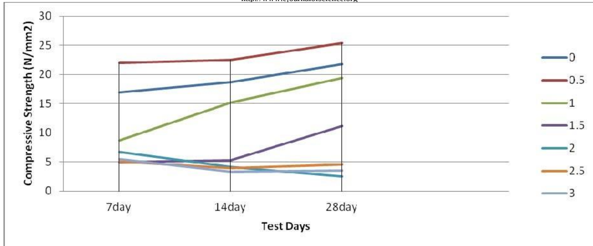
Graph 3: Compressive Strength (N/mm 2 )
