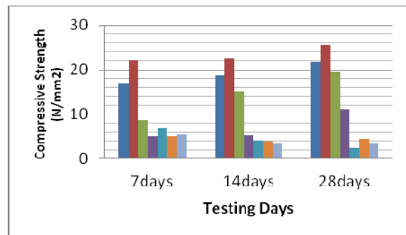
Fig 1: Compressive Strength (N/mm 2 )
