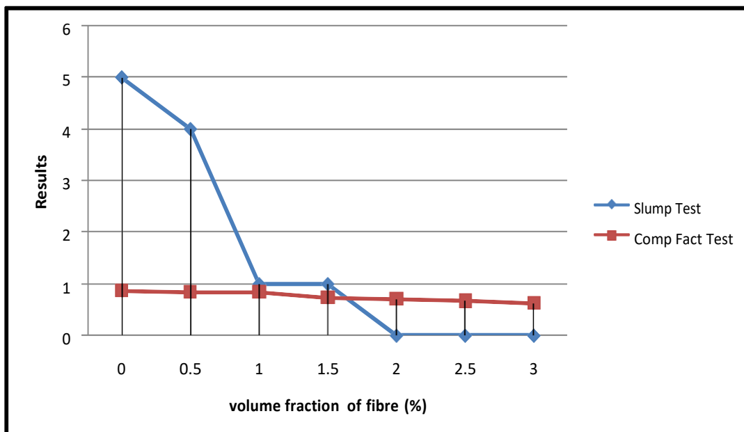
Graph 1: Workability Tests
