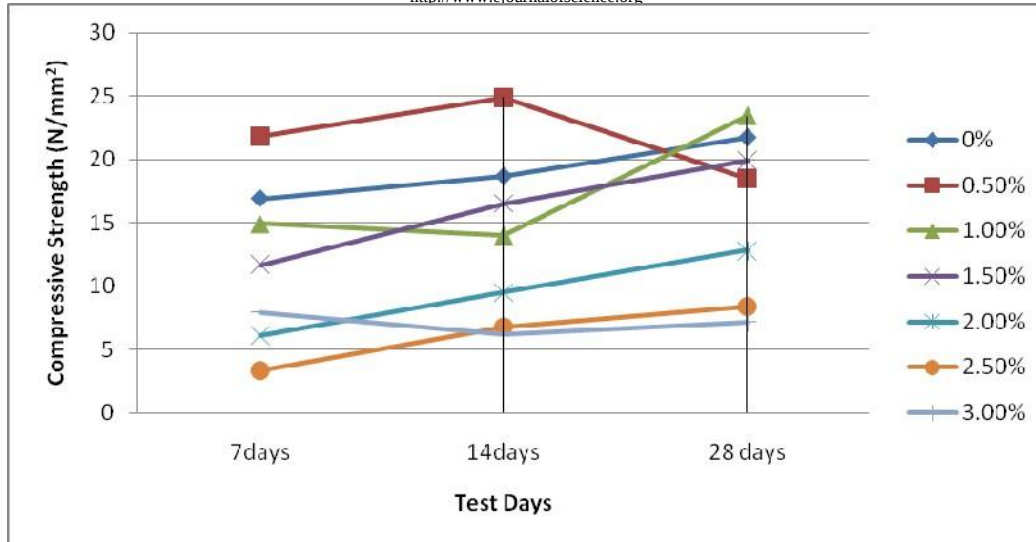
Graph 2: Compressive Strength at 7, 14 and 28 days
