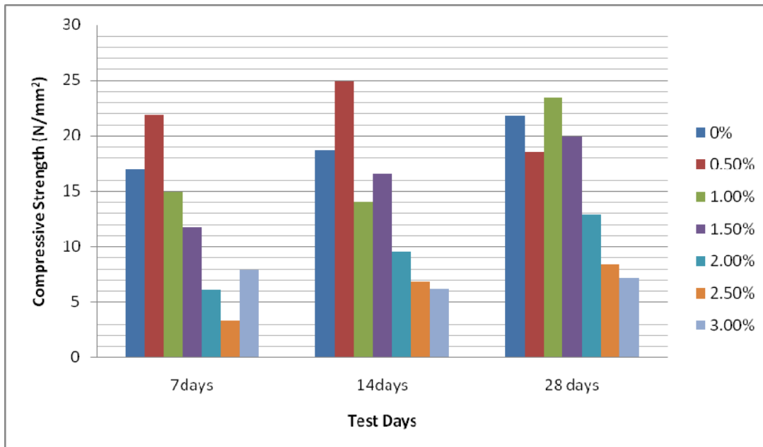
Fig 1: Compressive Strength at 7, 14 and 28 days
