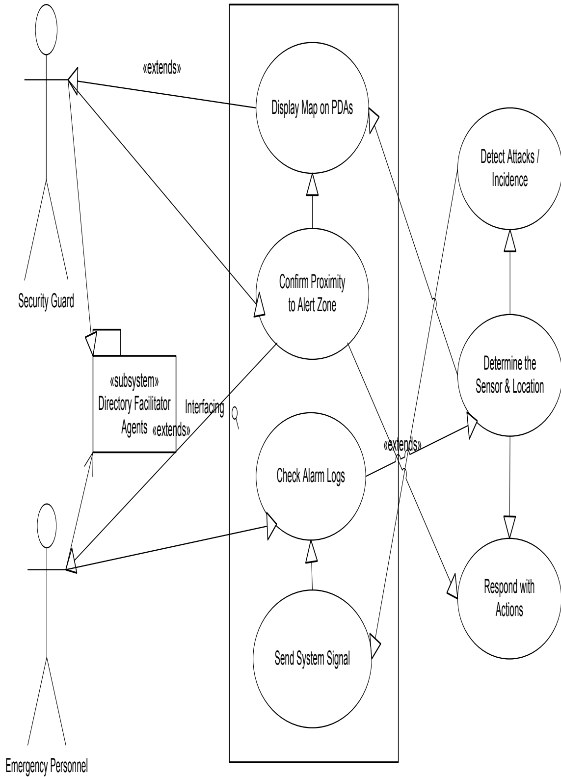
Fig. 2 A conceptual model of web-agent system in use-cases
