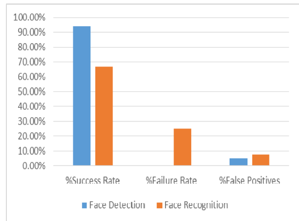
Fig. 9 Visualization graph for 50 live facial data
