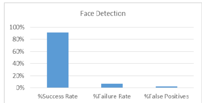
Fig. 10 Visualization graph for 20 static facial data
