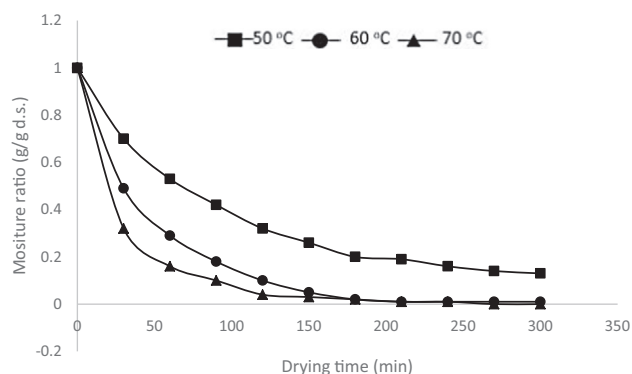
Fig. 1. Drying curves of 4 mm tomato slices at different temperatures.
