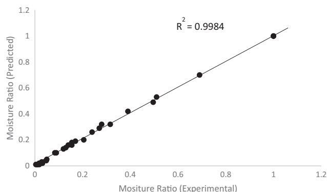
Fig. 3. Correlation between Page predicted and experimental moisture ratio.
