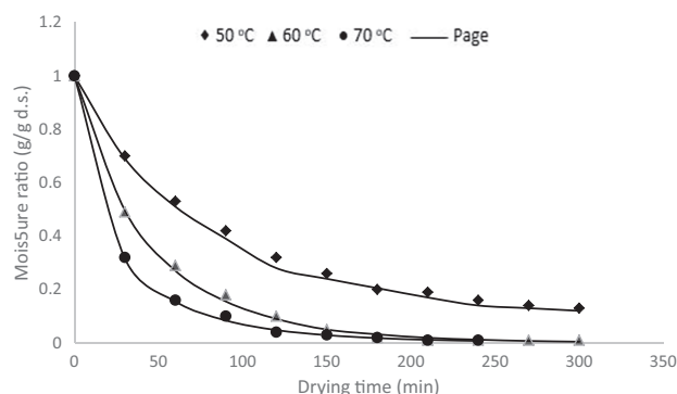
Fig. 2. Drying curves of experimental moisture ratio and Page model predicted moisture ratio of 4 mm tomato slices.
